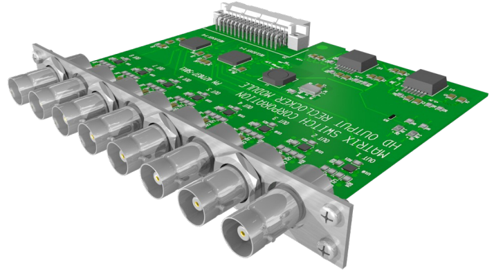
MSC-XD8TB - 8 Output SDI Video Reclocker Card
